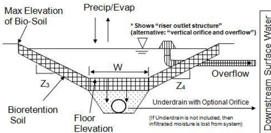
Revised Schematic
