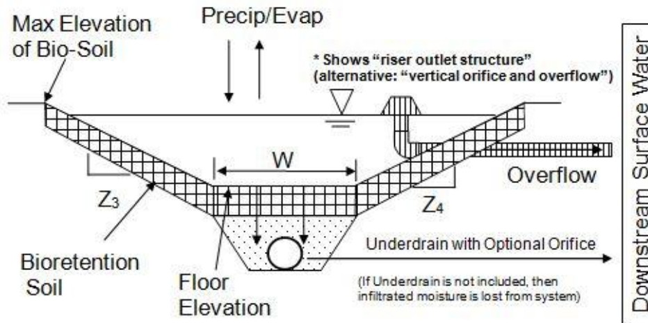
Revised Schematic
